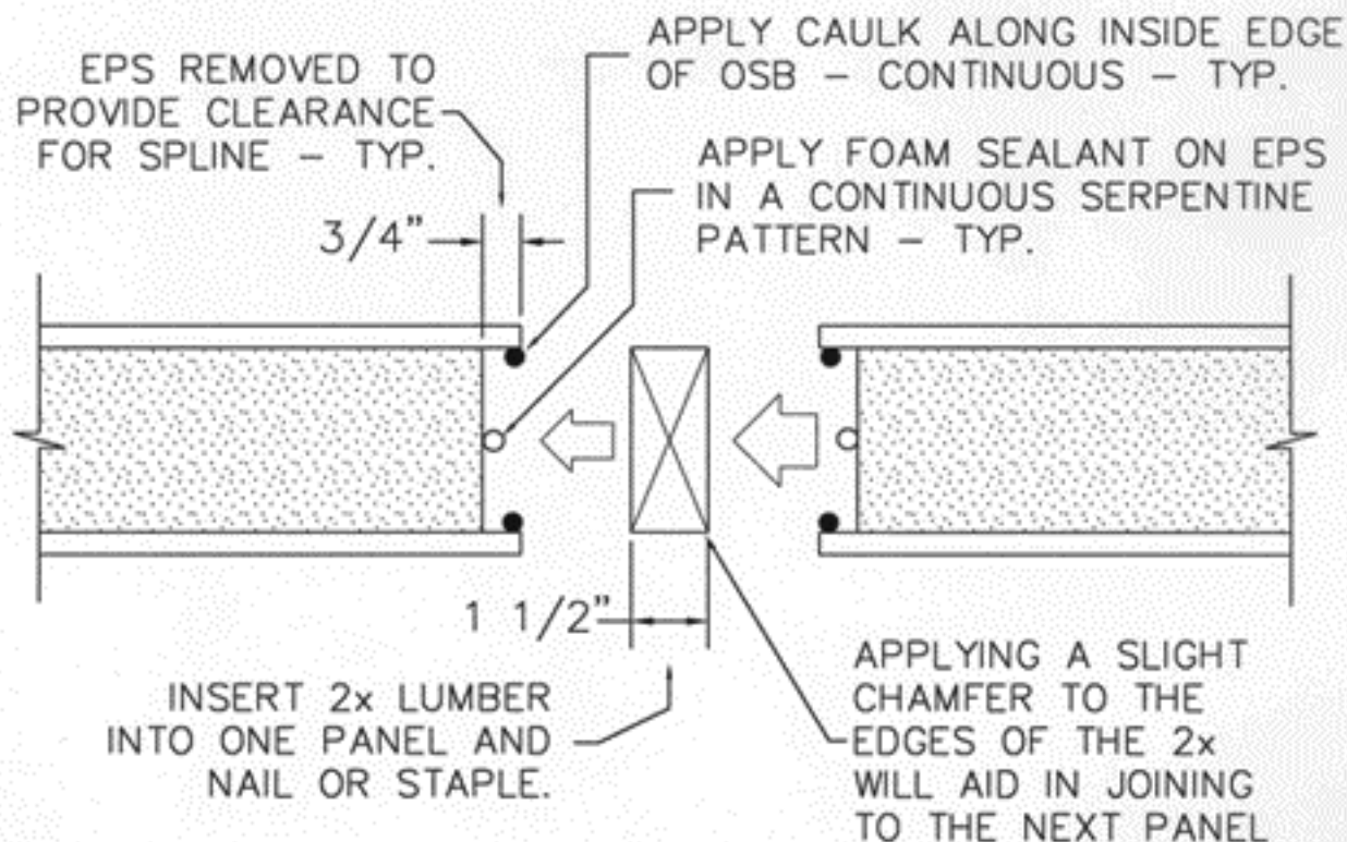
HORIZONTAL SECTION WALL OR ROOF PANELS BEFORE ASSEMBLY
