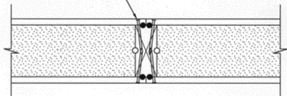
HORIZONTAL SECTION WALL OR ROOF PANELS ASSEMBLED
